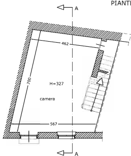
PIANO TERRA
